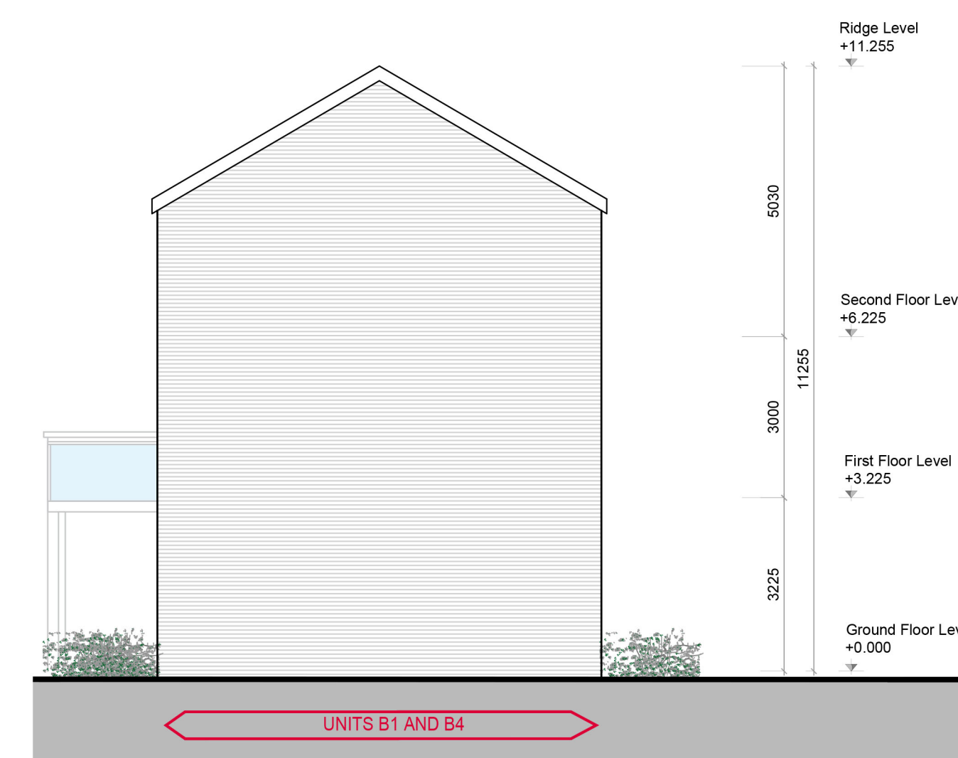
EAST ELEVATION
