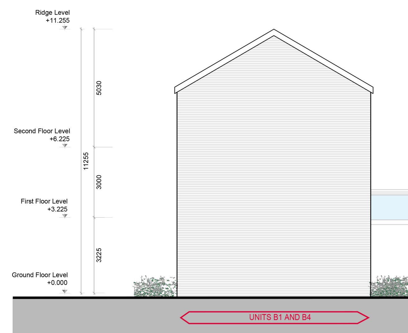
WEST ELEVATION
