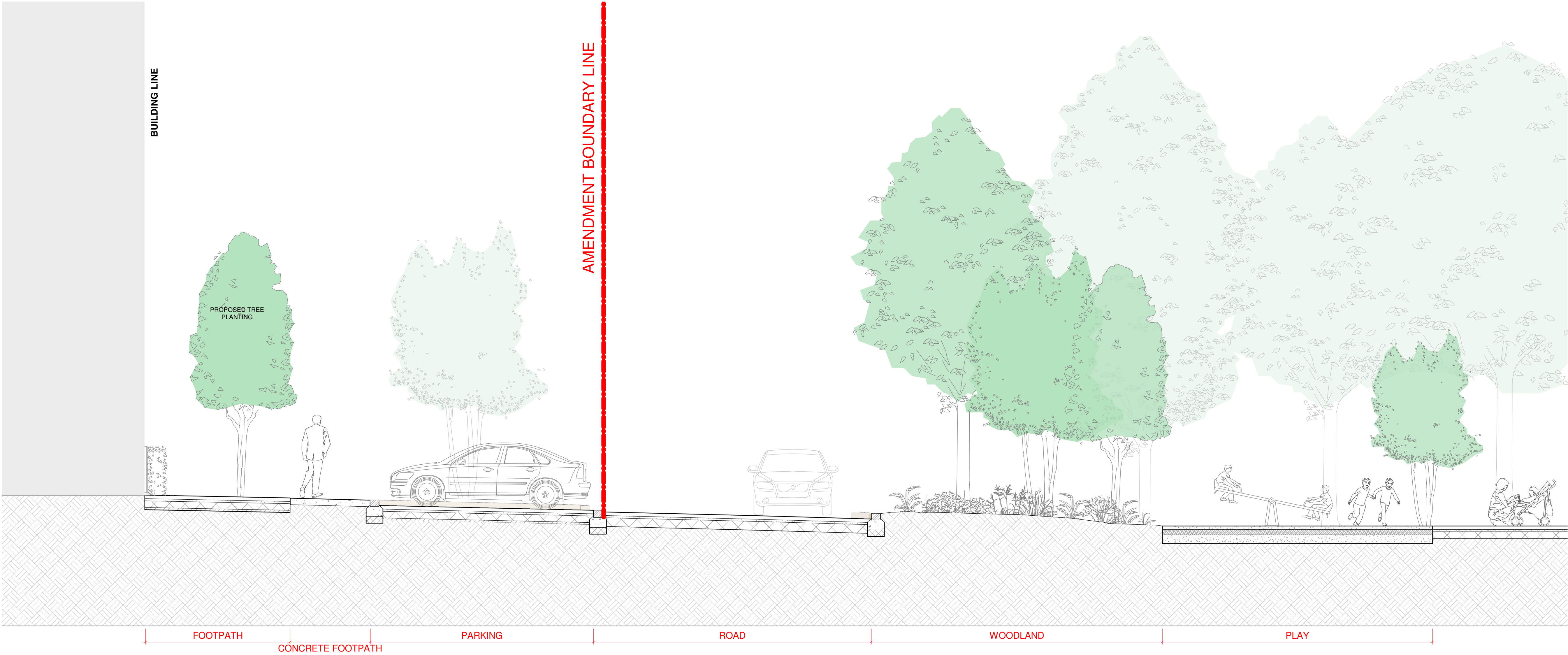
1 Neighbourhood Centre - Section 05 SCALE: 1 : 50 @A1
